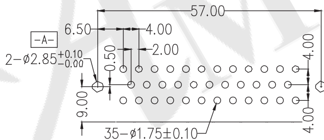
Recommended PCB Layout (Top Side) (PCB TOLERANCE ±0.05)
